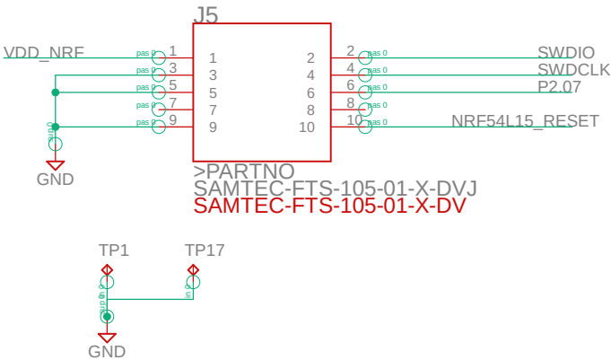
Debug In Connector
