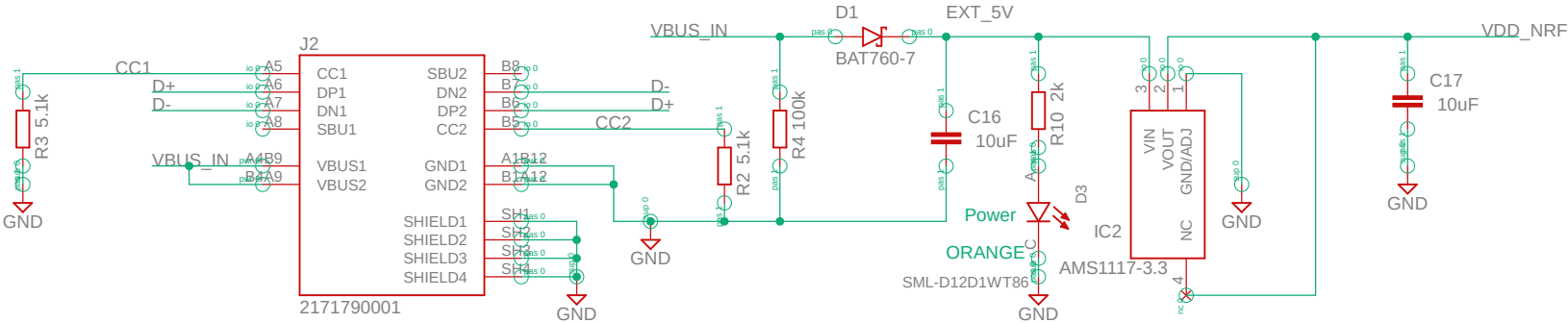
TypeC Connector
