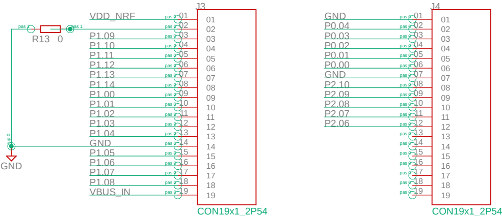
Debug 2.54mm GPIO Connector
