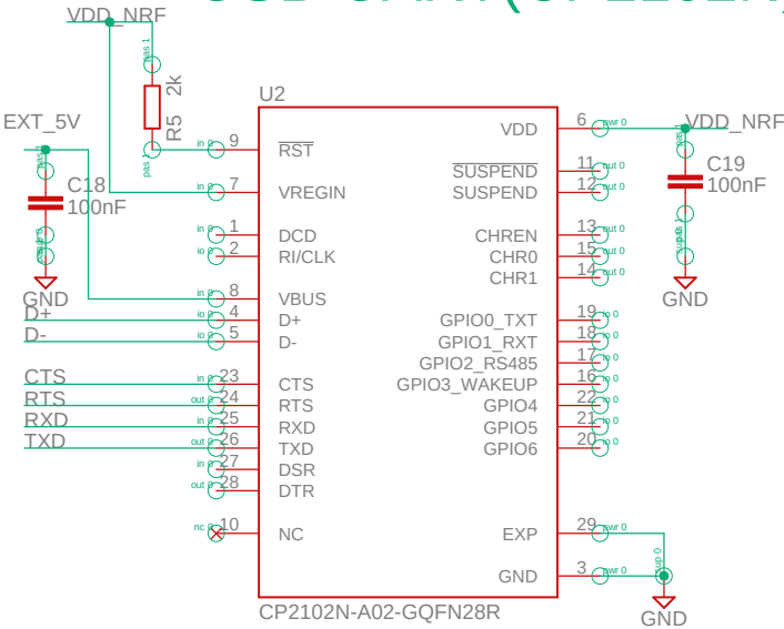
USB-UART(CP2102N)
